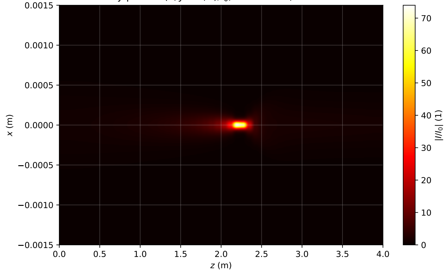
Intensity profile I(x, y = 0, z)/I_0 , P_{in}=1.3P_{cr} , artificial time
